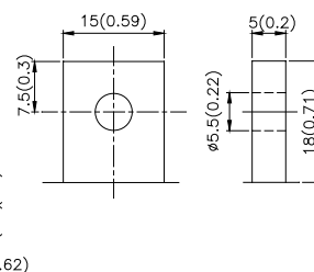
A Detail Drawing
