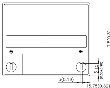
A Detail Drawing
